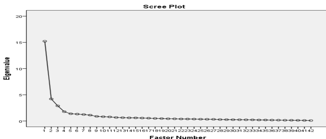
Figure 2. Scree Plot for TPACK Scale
